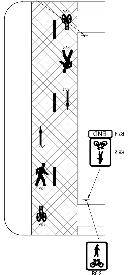
PLAN – APPROACH TO ROAD CROSSINGS FOR PATHS ADJACENT TO ROAD
