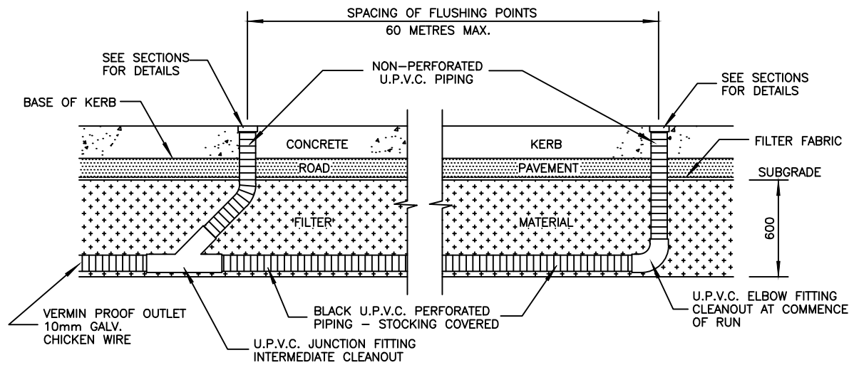
TYPICAL LONGITUDINAL SECTION
