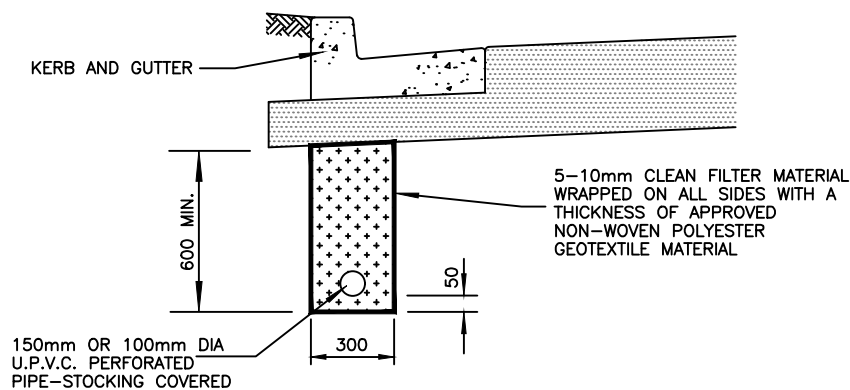
TYPICAL SECTION
