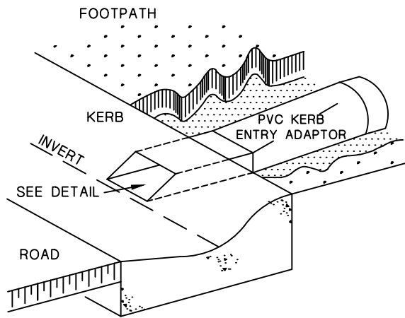
CASE 3 ROLLED KERB AND "ANGLE CUT" KERB ENTRY ADAPTOR
