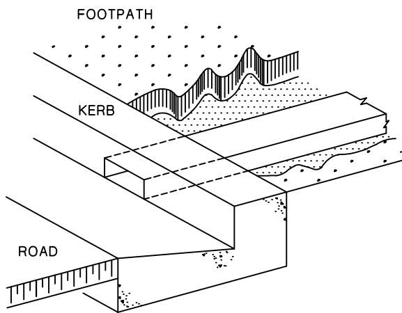
CASE 2 KERB ENTRY WITH RHS (100x200)
